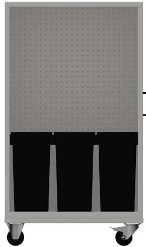
"Easy Clean" cleaning station Perforated rear panel (mounted) 3 waste bins made of polypropylene, 60 litres
